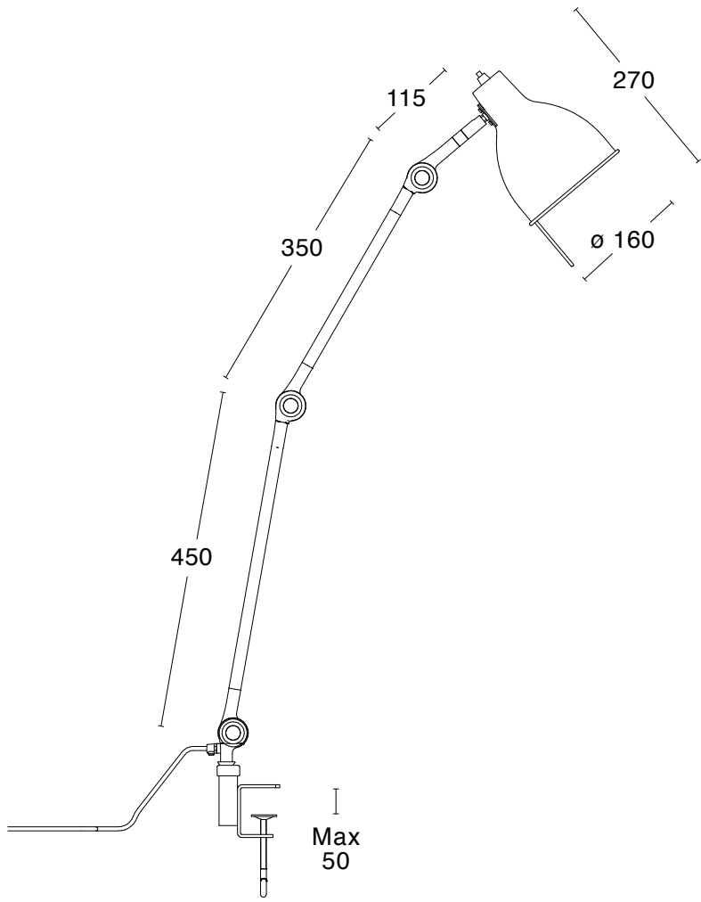
PJ65 - CLAMP
